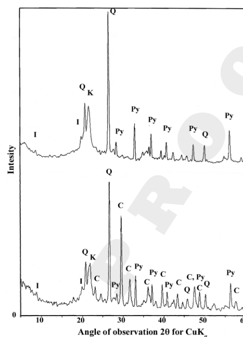
Fig. 1. XRD pattern of raw and HCl concentrate oil shale for the Aleksinac oil shale deposit. (Q: quartz, I: illite, K: cristobalite, Py: pyrite, C: calcite)
